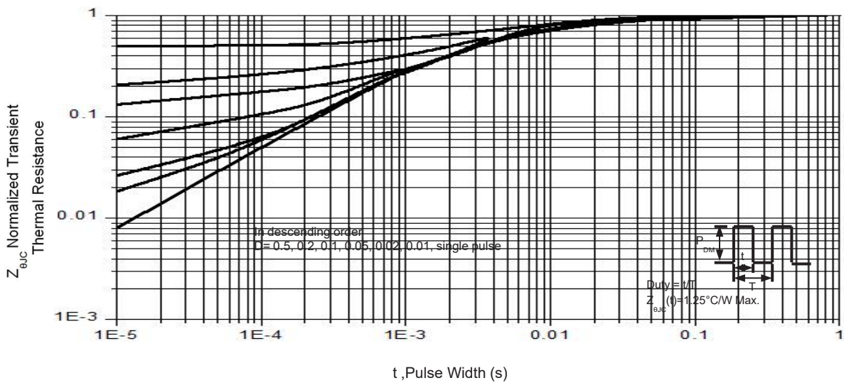
Figure 16. Transient Thermal Impedance, Junction to Case \zeta TO-220/TO-251/TO-252
