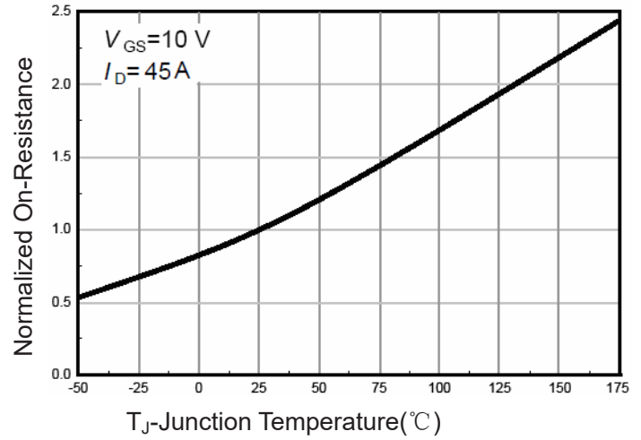
Figure 4 Rdson-Junction Temperature
