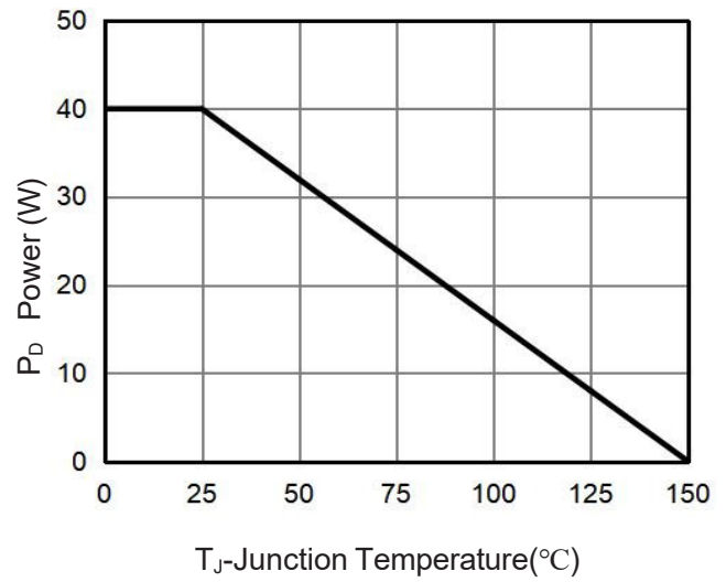
Figure 9 Power Dissipation
