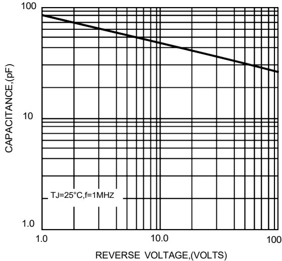
FIG.3-TYPICAL JUNCTION CAPACITANCE
