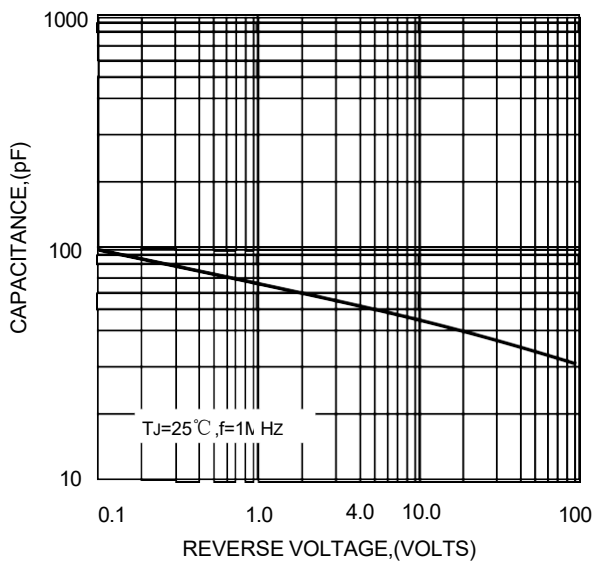
FIG.3-TYPICAL JUNCTION CAPACITANCE
