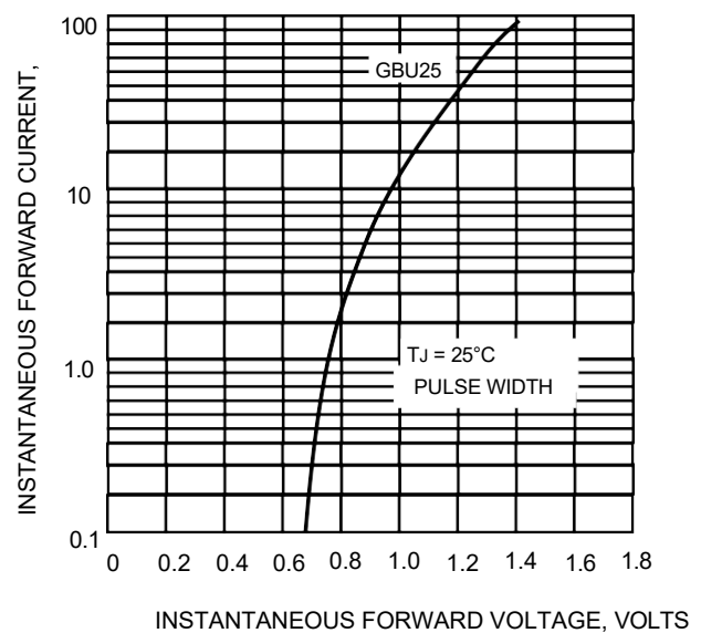
FIG.4-TYPICAL FORWARD CHARACTERISTICS
