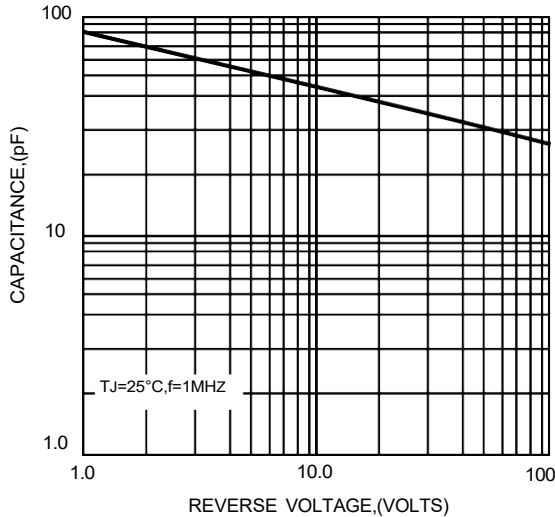
FIG.5-TYPICAL REVERSE CHARACTERISTICS
