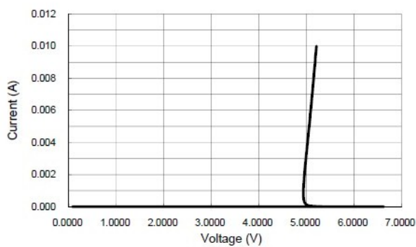
Fig 3 Voltage Sweeping
