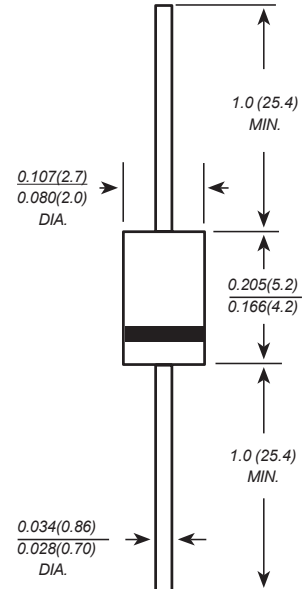
DO-41
