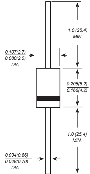
DO-41
