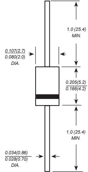
DO-41
