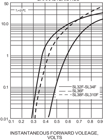
FIG. 3-TYPICAL INSTANTANEOUS FORWARD CHARACTERISTICS
