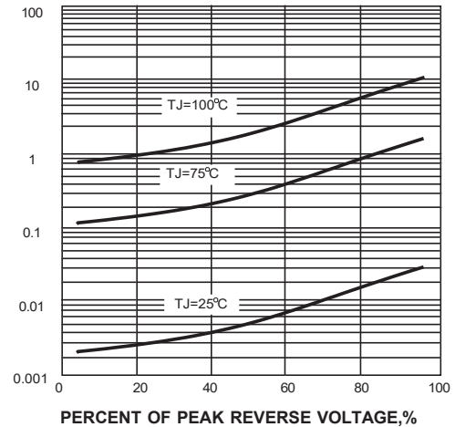
FIG. 4-TYPICAL REVERSE CHARACTERISTICS
