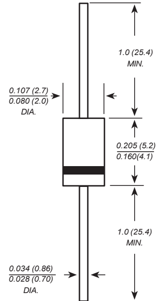
DO-41
