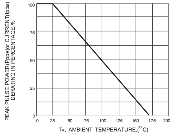
FIG. 2-PULSE DERATING CURVE
