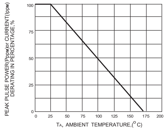
FIG. 2-PULSE DERATING CURVE
