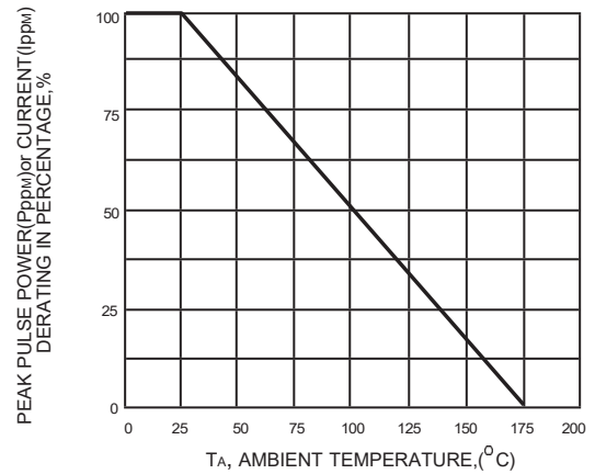
FIG. 2-PULSE DERATING CURVE
