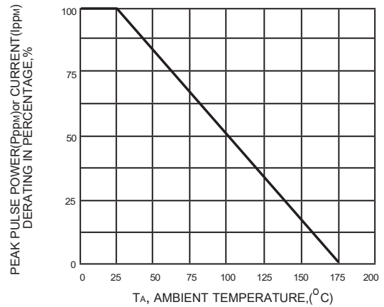
FIG. 2-PULSE DERATING CURVE
