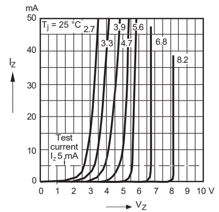
Fig. 14 - Breakdown Characteristics
